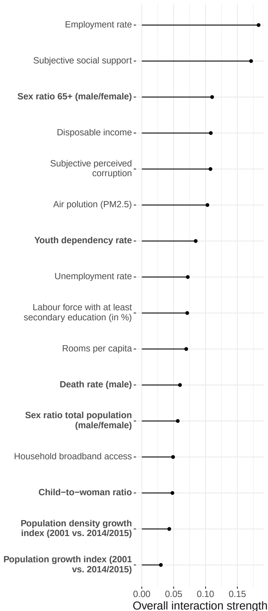
Random Forest
