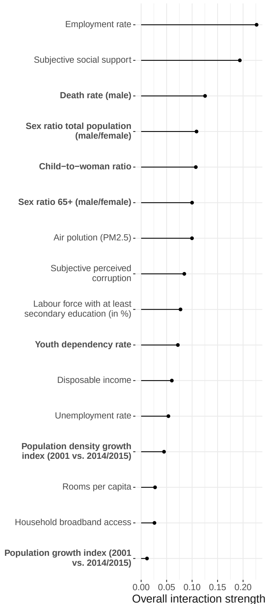
XGBoost
